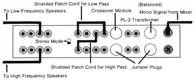
CS-1200 PATCH DIAGRAM 5 Biamp Operation Balanced Low Z Input (Monaural Signal)
